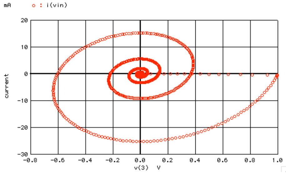
Graph 4 - tran1: X-Y Plot example (CDHW Version)
