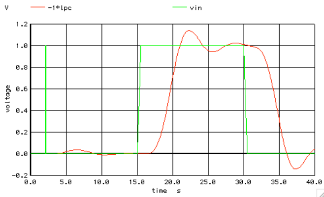
Graph 33 - tran34: Butterworth_6P_State_Variable
