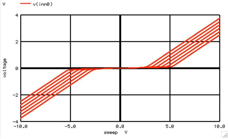
Graph 43 - dc50: OTA_DEADZONE
