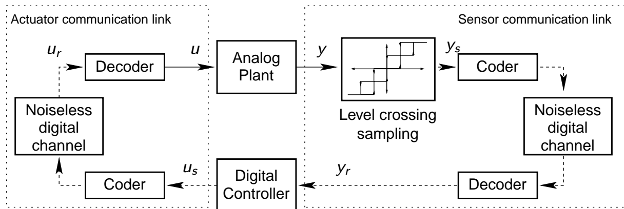
Figure 1: Event-driven sampled-data scheme for feedback stabilization over digital channels
