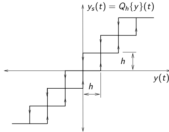
Figure 3: Quantizer with hysteresis, y_s(t) = Q_h\{y\}(t)
