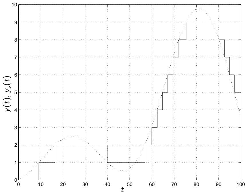
Figure 2: Event-driven sampling/quantization
