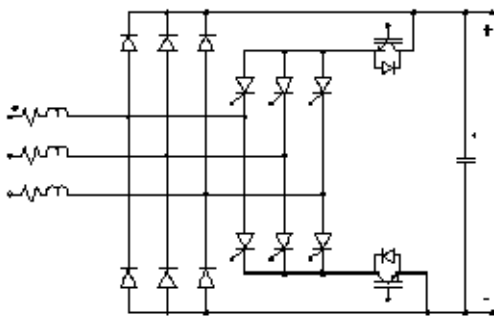
Fig 4: SCR Bridge with turn-off switches
