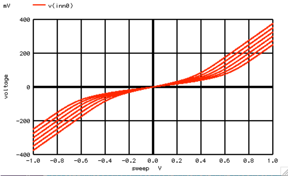
Graph 39 - dc46: OTA_SPRINGHARDEN
