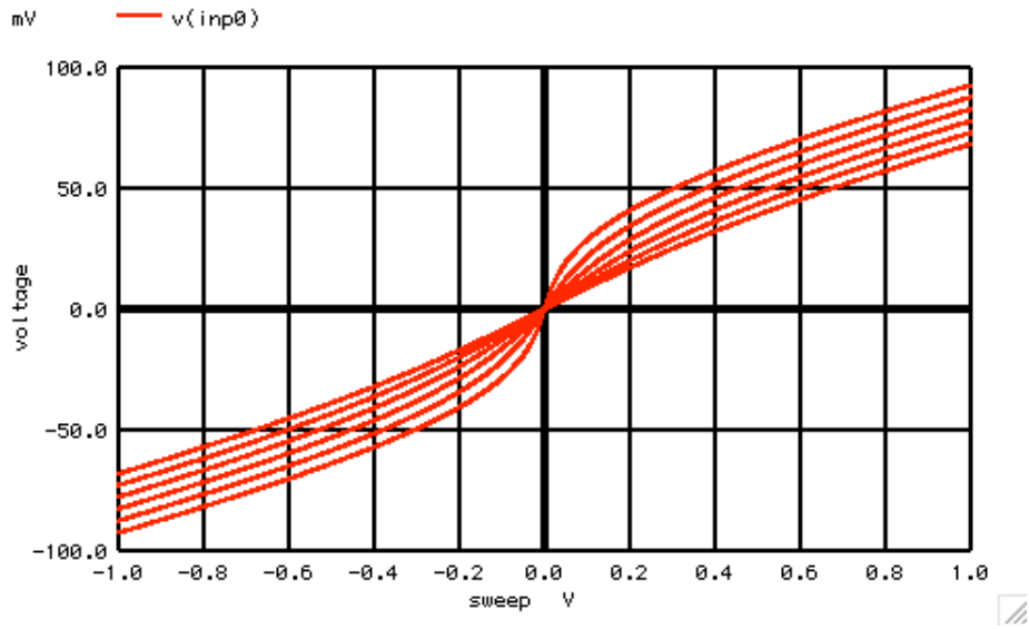
Graph 40 - dc47: OTA_Preload
