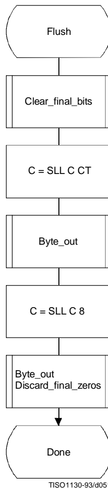
Figure D.13 – Flush procedure
