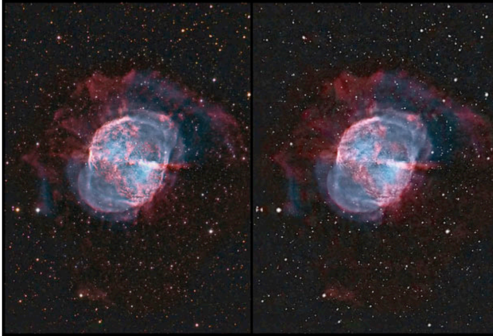
The Dumbbell Nebula, M27, which is about 1,250 light years away in the constellation Vulpecula
